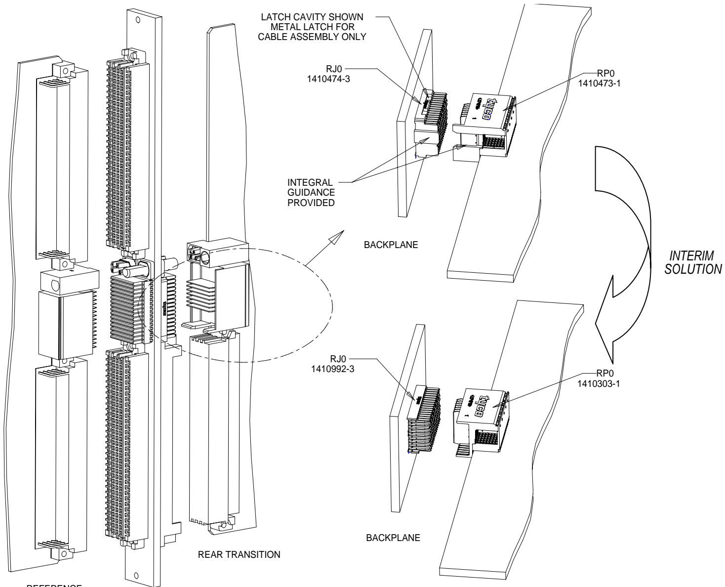
VITA 41 VXS VMEbus Switched Serial Payload Rear Transition Module
