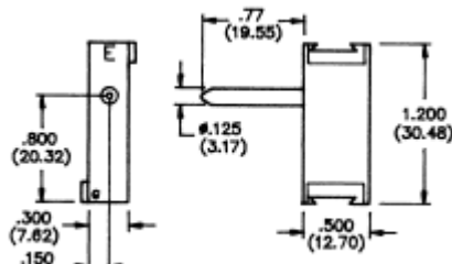
Guide Pin Part Number 1648505-1
