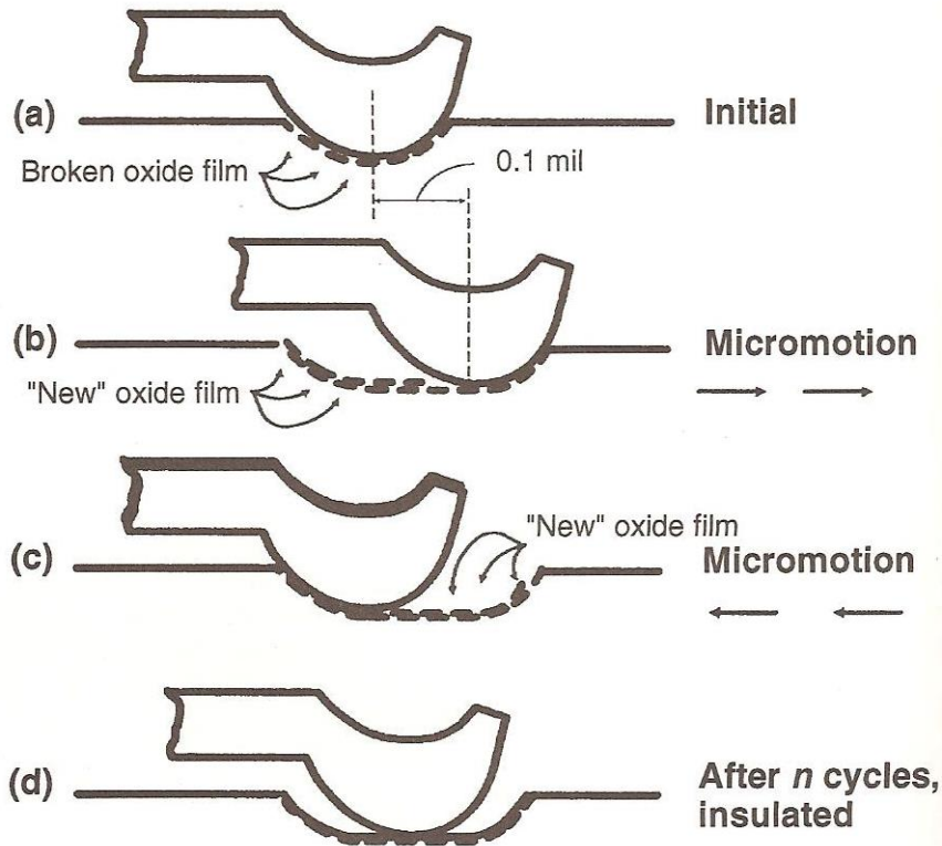
Figure 5. Fretting corrosion from micromotions
