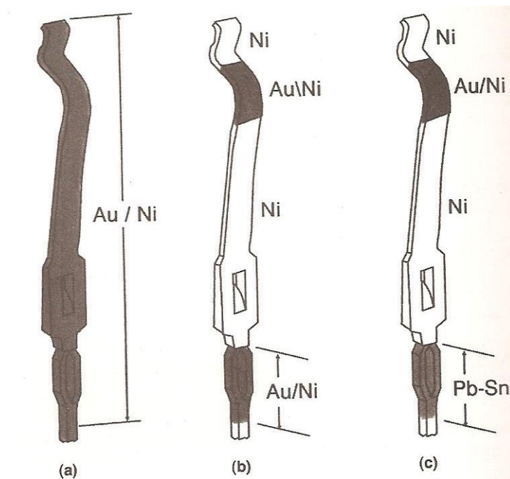
Figure 3. Approaches to plating to reduce gold without decreasing performance.
