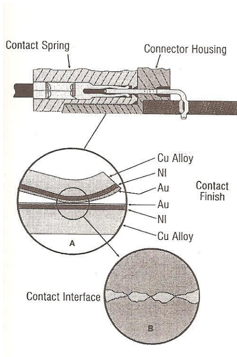
Figure 2. A separable connection includes a housing, contact, and contact plating.
