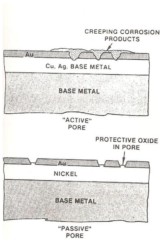
Figure 4. Nickel prevents corrosion from migrating through micropores from the base material through gold plating to the surface.
