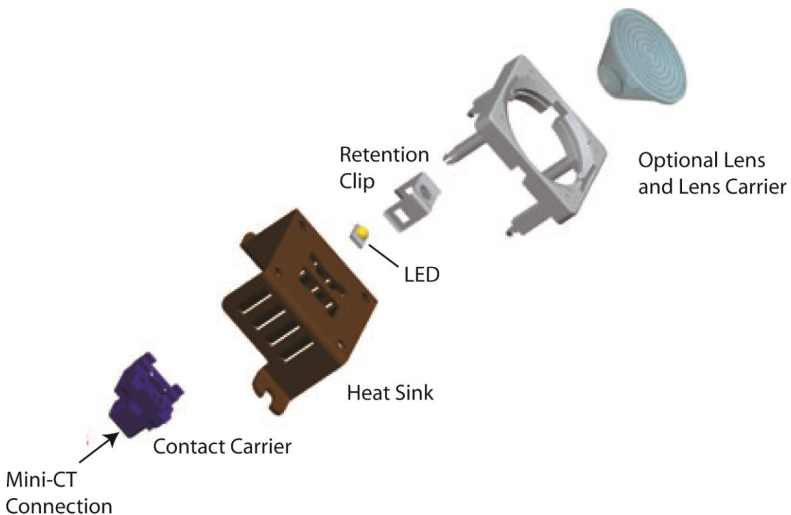
Figure 7. High-intensity LED holder combines thermal, mechanical, and electrical management into a single, easy-to-use system.
