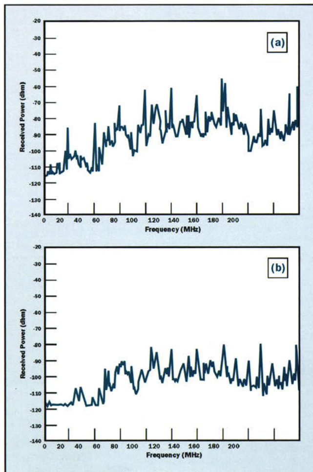
Figure 1. Illustration of radiated emission measurements in a MSC. (a) original emission of a computing product; (b) emission after product modification.
