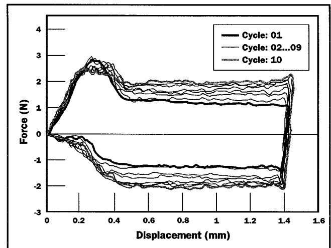
Figure 3. Force versus displacement for the first ten insertion/withdrawal cycles measured on non-lubricated contacts.
