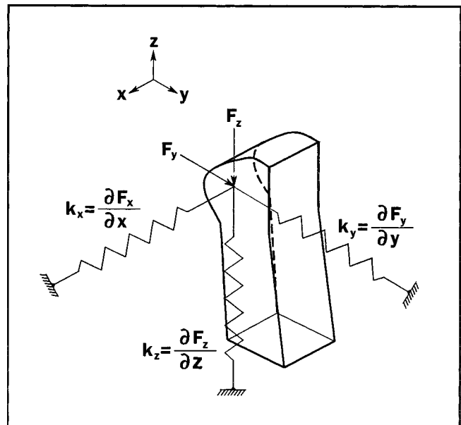
Figure 2. Schematic of a spring-supported contact region.
