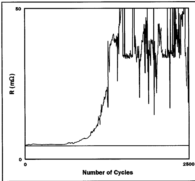
Figure 6. Changes of contact resistance versus number of cycles measured on contacts without position spring.
