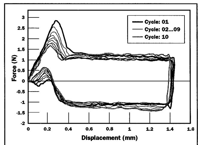
Figure 4. Force versus displacement for the first ten insertion/withdrawal cycles measured on lubricated contacts.
