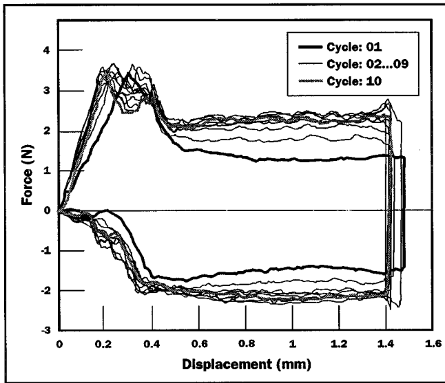
Figure 5. Force versus displacement for the first ten insertion/withdrawal cycles measured on contacts without position spring
